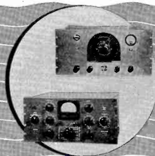
15. MEASURING EQUIPMENT —The RCA, 68-B Audio Oscillator and the RCA, 69-C Distortion Meter are universally used for determining the frequency response and distortion characteristics of broadcast installations.
